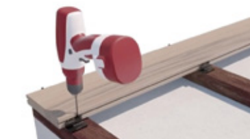
05 The fifth step Install screws
