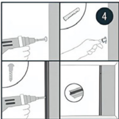
④ If you use expansion screws, you need to drill holes in advance and mark the drilling positions with a pencil. If you use an air nail gun, you do not need to drill holes in advance.
